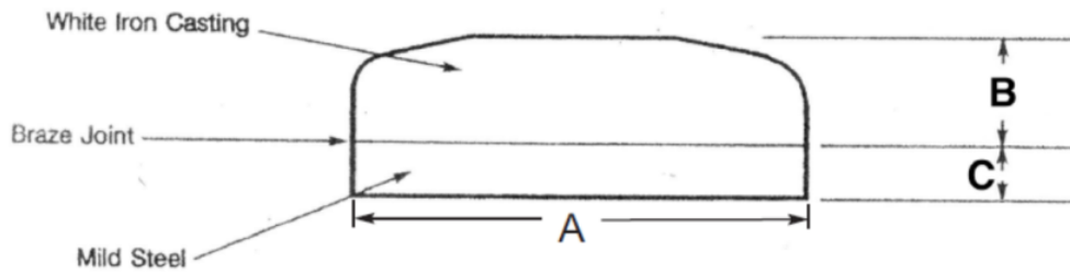
WEAR BUTTONS (WHITE IRON)
