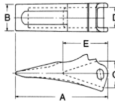
CAT® STYLE RIPPER TOOTH AND SHANK for 951, 955, 140, 140G
