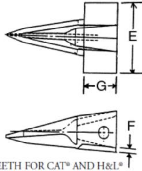
FLYING TIGER® AND WING TIP STYLE TEETH FOR CAT® AND H&L® (Patented)
