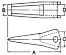
Type 1- Centerline Ripper Tooth
